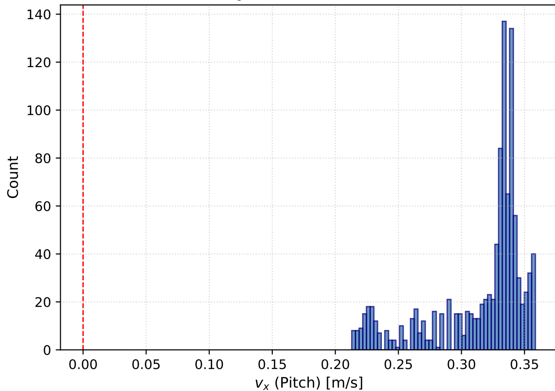
Pitch Velocity Commands ( \sigma=0.0378 m/s)
